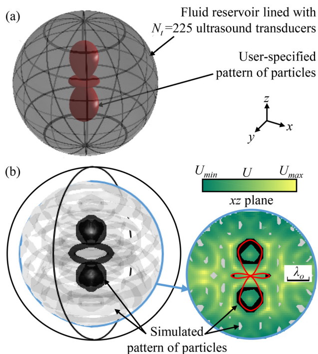
FIG. 5. (a) User-specified electron d_{z^2} orbital pattern of particles (red) prescribed in a spherical fluid reservoir and (b) simulated pattern of particles (gray) achieved by solving the 3D inverse problem. Inset images show a cross section of the user-specified (red) and simulated (gray) patterns overlaying the radiation potential U (green) and a scale bar indicating the wavelength \lambda_0 .
