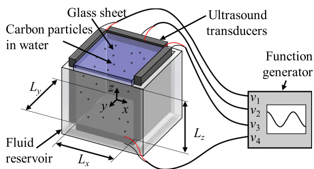
FIG. 2. Schematic of the fluid reservoir with L_x = L_y = L_z = 12.75 mm = 12.75\lambda_0 , containing carbon particles dispersed in water, and showing the ultrasound transducers driven with operating parameters (amplitude and phase) v_1, v_2, v_3 , and v_4 , respectively.
