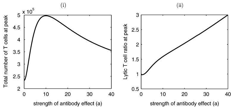
FIG. 3. Antibody effects on the total number of T cells ( T_2 + T_{2c} + T_4 + T_{4c} ) and the lytic T-cell ratio ( (T_4 + T_{4c})/(T_2 + T_{2c}) ) in the absence of cross-reactive T cells ( \sigma_j = 0 ). (i) Total number of CD8^+ T cells at the peak of infection. (ii) The lytic T-cell ratio at peak: ratio between the number of T cells against lytic infection ( T_4 ) and the number of T cells against latent infection ( T_2 ), evaluated at the peak of infection. Parameter values are shown in Tables 1 and 2.
