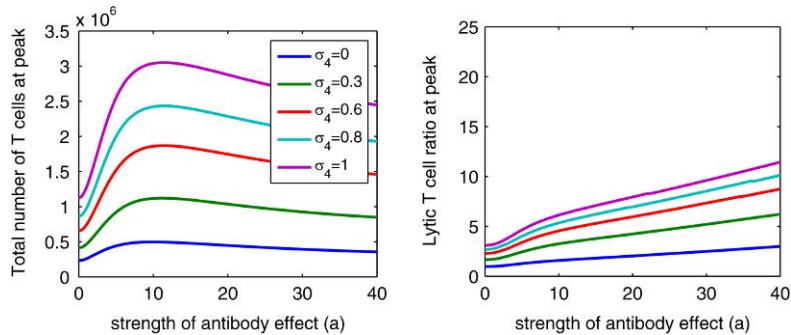
FIG. 5. The effects of both latent and lytic cross reactive T cells ( \sigma_j > 0 ) on the total number of T cells and the lytic T-cell ratio during primary infection as a function of the strength of the antibody effect ( a ). The five different degrees of cross-reactive responses are shown in the plots. For each level of \sigma_4 , \sigma_2 = 0.2\sigma_4 . We set \chi_2 = 0.5 and \chi_4 = 0.1 . Other parameter values are shown in Tables 1 and 2.
