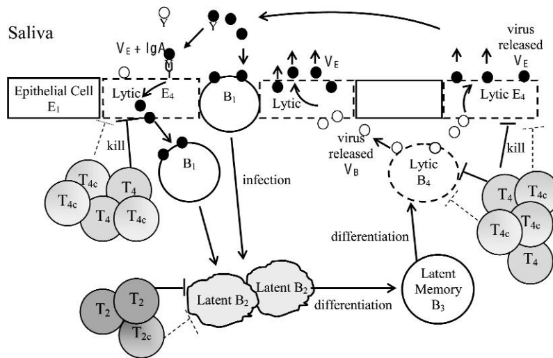
FIG. 1. Model of EBV infection of B cells and epithelial cells. Antibodies like IgA can shift the viral target from B cells to epithelial cells. Activation of cross-reactive memory T cells ( T_{2c} , and T_{4c} ) that are not efficient in killing infected cells may contribute to the pathology of IM.
