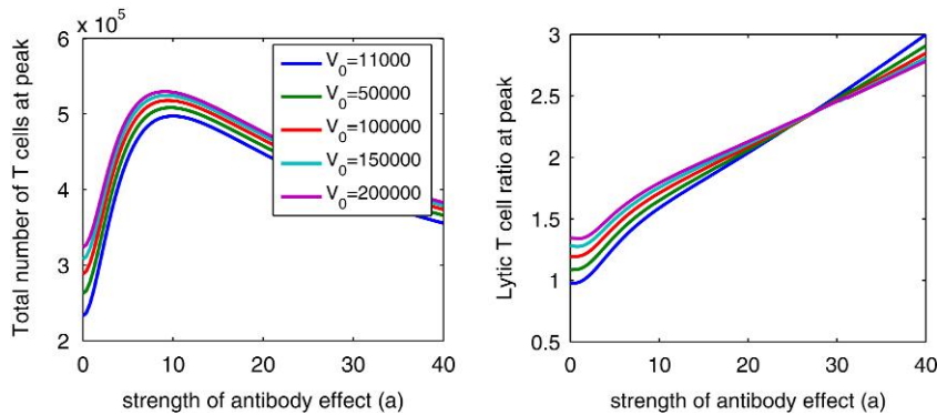
FIG. 6. The effect of initial viral load ( V_0 ) on the total number of T cells and the lytic T-cell ratio during primary infection as a function of the strength of the antibody effect ( a ). We set \sigma_j = 0 which represents no cross-reactive T-cell response. Other parameter values are shown in Tables 1 and 2.
