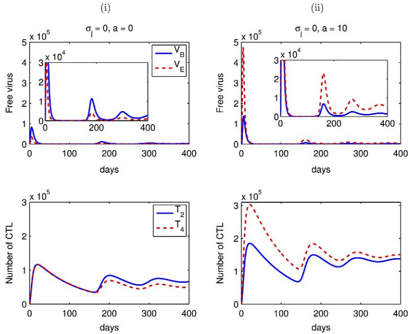
FIG. 2. Dynamics of viruses and T cells in the case of no cross-reactive T-cell responses ( \sigma_j = 0 ). (i) Without antibody effect ( a = 0 ). (ii) With antibody effect ( a = 10 ). The insets show the level of persistent virus for the two cases. Parameter values used are shown in Tables 1 and 2.
