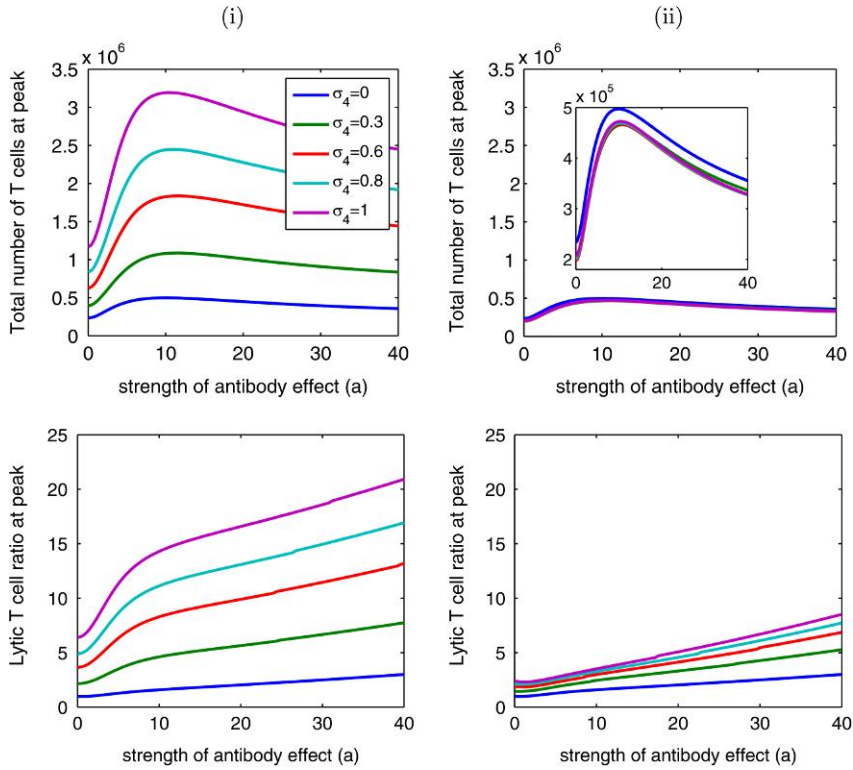
FIG. 4. The effects of cross-reactive T-cell responses to viral lytic proteins ( \sigma_4 > 0 ) on the total number of T cells and the lytic T-cell ratio during primary infection as a function of the strength of the antibody effect ( a ). The five different degrees of cross-reactive responses are shown in each plot. (i) Left column: low efficiency of cross-reactive lytic T cells in killing infected cells ( \chi_4 = 0.1 ). (ii) Right column: cross-reactive T cells are as efficient as specific T cells in killing infected cells ( \chi_4 = 1 ). Other parameter values are shown in Tables 1 and 2.
